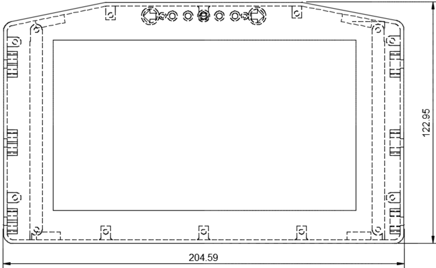
BTI 7" Dash Dimensions in mm
